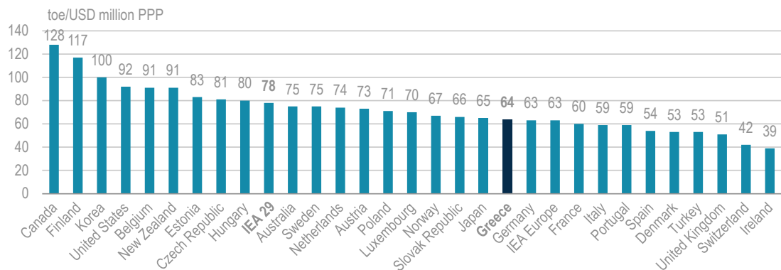
Figure 7.4 TFC in IEA member countries, 2015
